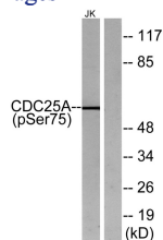
Western Blot analysis of Jurkat cells using Phospho-Cdc25A (S75) Polyclonal Antibody
