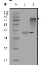
Western Blot analysis using Cytokeratin 19 Monoclonal antibody against truncated KRT19-His recombinant protein (1) and full-length KRT19(aa1-400)-hIgGFc transfected CHO-K1 cell lysate(2).
