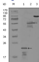
Western Blot analysis using ErbB-3 Monoclonal antibody against truncated Trx-ERBB3 recombinant protein (1) MBP-ERBB3 (aa1175-1275) recombinant protein (2) and truncated ERBB3(aa665-1342)-hlgGfC transfected CHO-K1 cell lysate (3).
