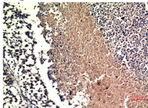
Immunohistochemical analysis of paraffin-embedded Human Lung Carcinoma Tissue using PTEN Mouse Monoclonal antibody diluted at 1:200.
