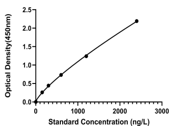
E2071Hu, Human M-AChR M1 Standard Curve
